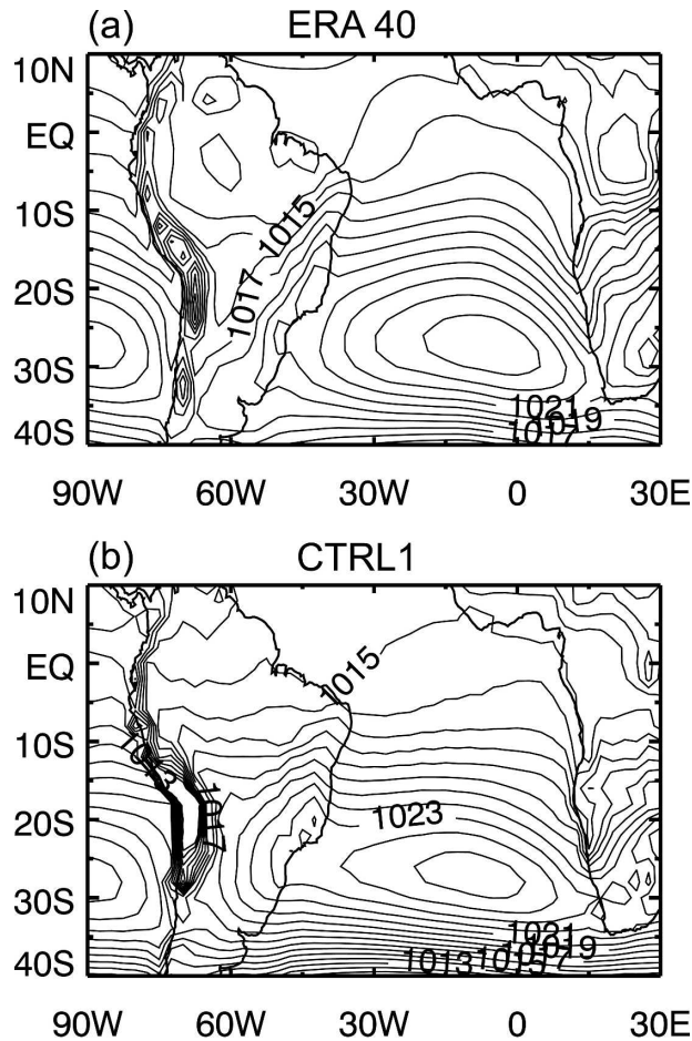
FIG. 1. SLP in July (long-term mean) for (a) ERA-40 and (b) CTRL1 (contour interval is 1 hPa). The anticyclone in CTRL1 is rather elongated in the zonal direction and not as well confined over the ocean as its counterpart in the reanalysis data.
