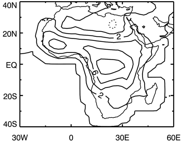
FIG. 10. Skin temperature difference (K) between PAD and CTRL1 for July.
