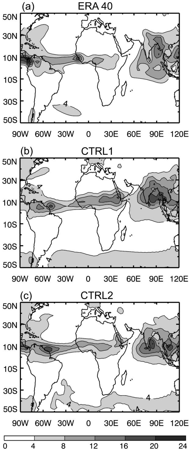
FIG. 4. Precipitation ( \text{mm day}^{-1} ) in July for (a) ERA-40, (b) CTRL1, and (c) CTRL2. The separation between African and Asian monsoon precipitation is much clearer in ERA-40 than in CTRL1.
