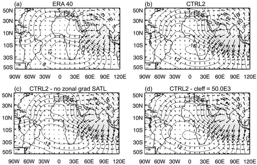
FIG. 12. Velocity potential and divergent wind in July for (a) ERA-40, (b) CTRL2, (c) an experiment in which the zonal gradient of SST is removed in the South Atlantic, and (d) an experiment with modified gravity wave drag coefficient.
