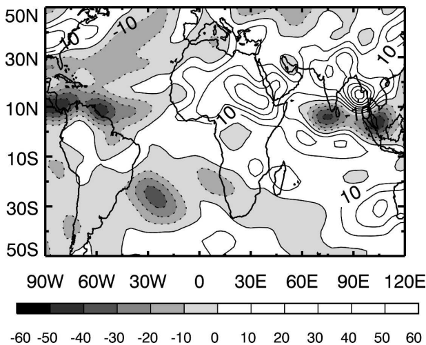
FIG. 13. As in Fig. 12 but for SLP.
