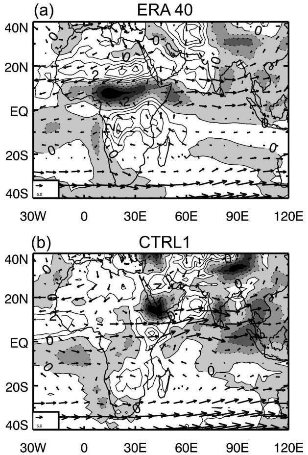
FIG. 5. Divergence ( 1 \text{ s}^{-1} \times 10^{-6} ) and horizontal wind at 700 hPa in July for (a) ERA-40 and (b) CTRL1. The reference vector in the lower left-hand corner shows 5 \text{ m s}^{-1} . Negative values are shaded.
