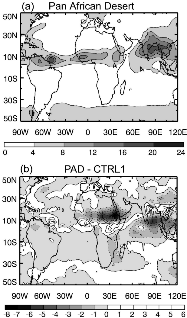
FIG. 9. Precipitation ( \text{mm day}^{-1} ) in July for (a) PAD and (b) the difference PAD - CTRL1. The altered land surface conditions in PAD reduce the excessive maximum over the Ethiopian highlands seen in CTRL1 and also produce a better separation between African and Asian monsoon precipitation.
