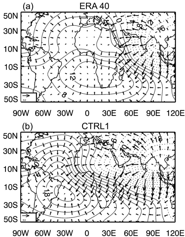
FIG. 2. Upper-level (200 hPa) divergent wind (vectors) and velocity potential (contours, \text{m}^2 \text{s}^{-1} \times 10^{-6} ) in July for (a) ERA-40 and (b) CTRL1. Negative contours are dotted. The reference vector in the lower left corner of each panel shows 5 \text{ m s}^{-1} . The upper-level divergence associated with the Asian summer monsoon extends much farther to the west in CTRL1 than in ERA-40. Consequently, divergence over the South Atlantic is shifted to the west in CTRL1.
