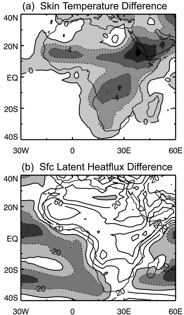
FIG. 6. (a) Ground temperature difference between CTRL1 and ERA-40 in July. CTRL1 features a cold bias over most of Africa. (b) As in (a) but for surface latent heat flux. The contour interval is 20 \text{ W m}^{-2} .
