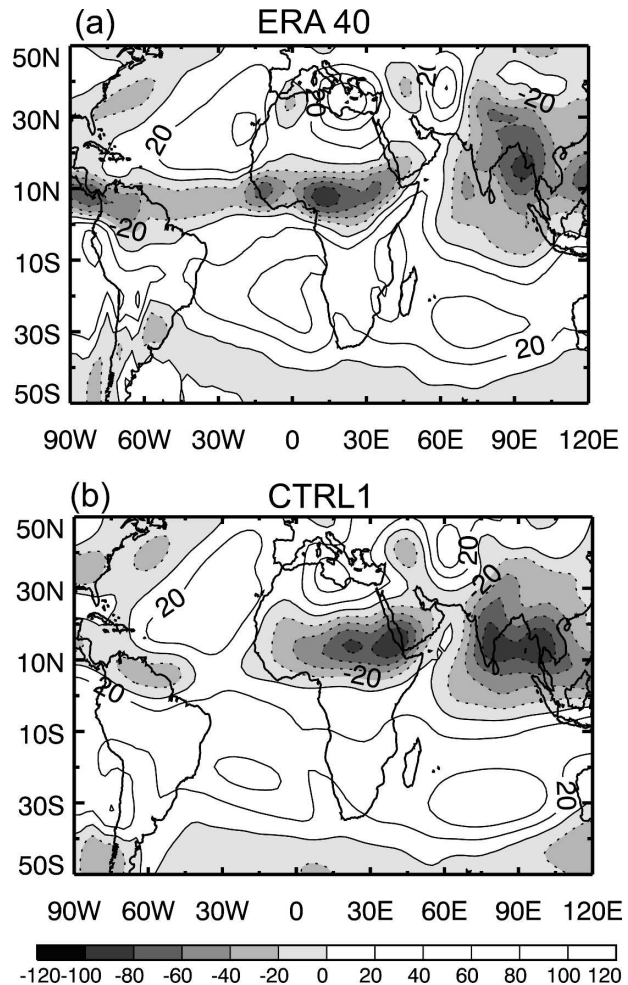
FIG. 3. Vertical p -velocity [ \text{hPa day}^{-1} ] at 500 hPa in July for (a) ERA-40 and (b) CTRL1. Negative values are shaded. This figure shows the lack of separation between African and Asian convection and a westward shift in subsidence over the South Atlantic. While ERA-40 places the maximum subsidence at around 0^\circ , CTRL1 shifts it to 20^\circ\text{W} .
