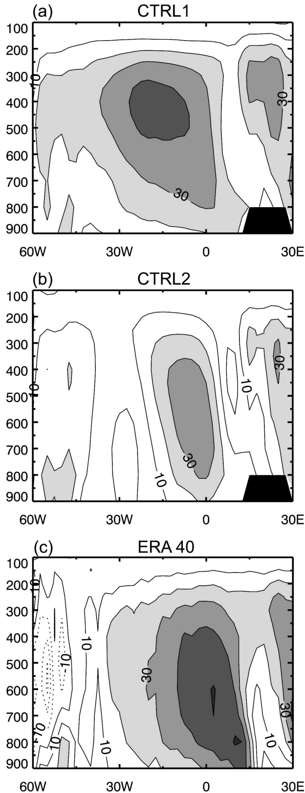
FIG. 14. Vertical p -velocity ( \text{hPa day}^{-1} ) in July averaged between 30^\circ and 20^\circ\text{S} in (a) CTRL1, (b) CTRL2, and (c) ERA-40. Values greater than +20 \text{ hPa day}^{-1} are shaded.
